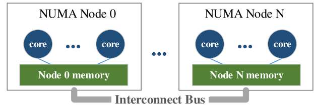
Fig. 4. NUMA topology.
